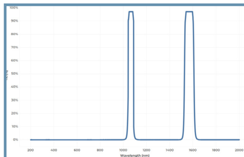
Dual-band coatings
